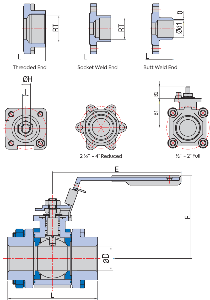
Dimensions(mm)
