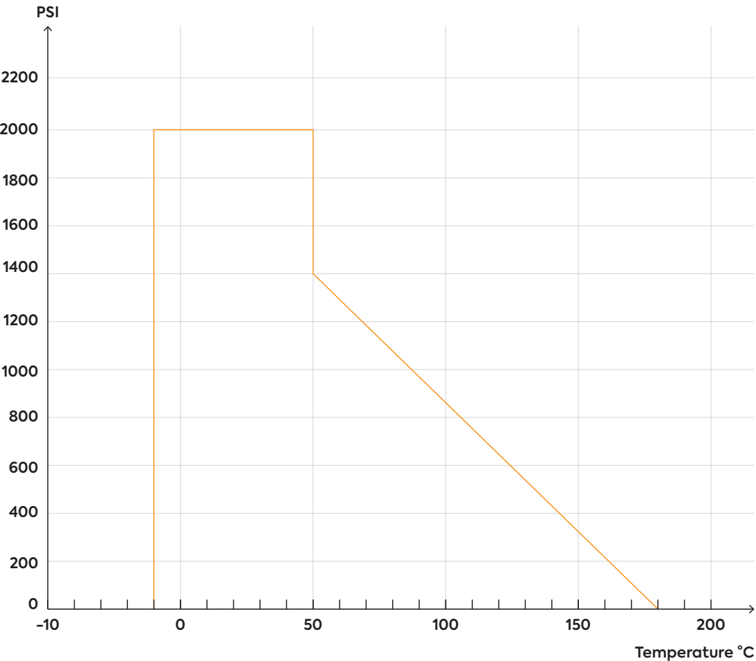
Pressure/Temperature Ratings
