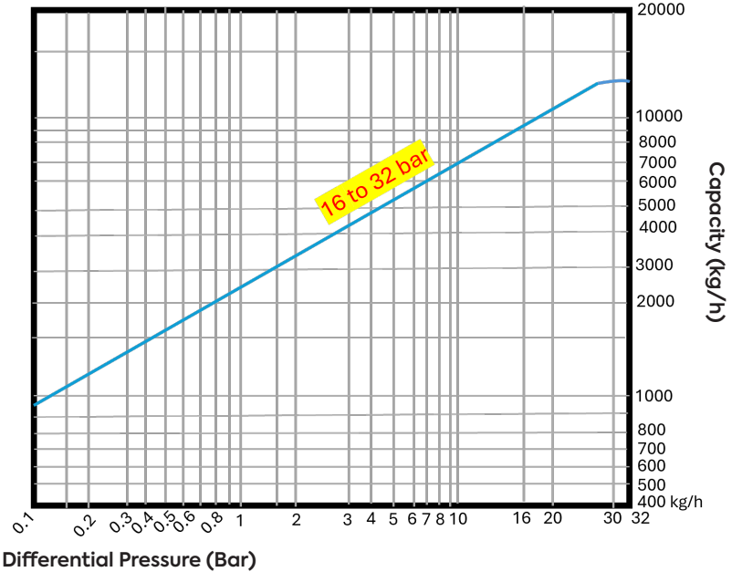
Displacement Curve
