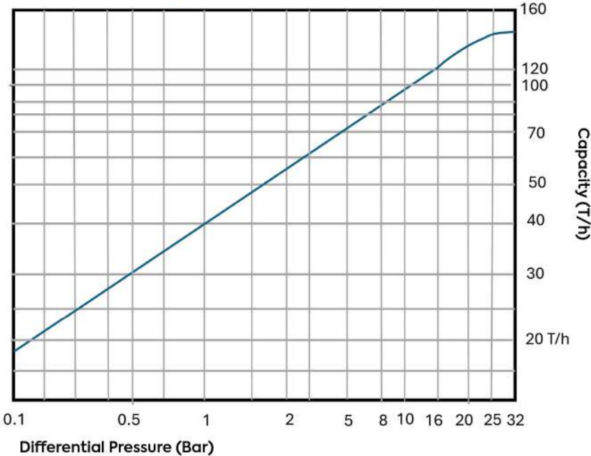
Displacement Curve
