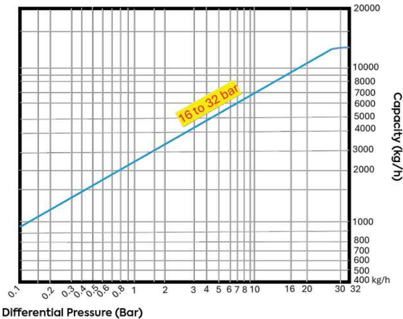
Displacement Curve
