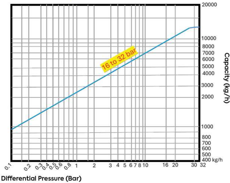
Displacement Curve
