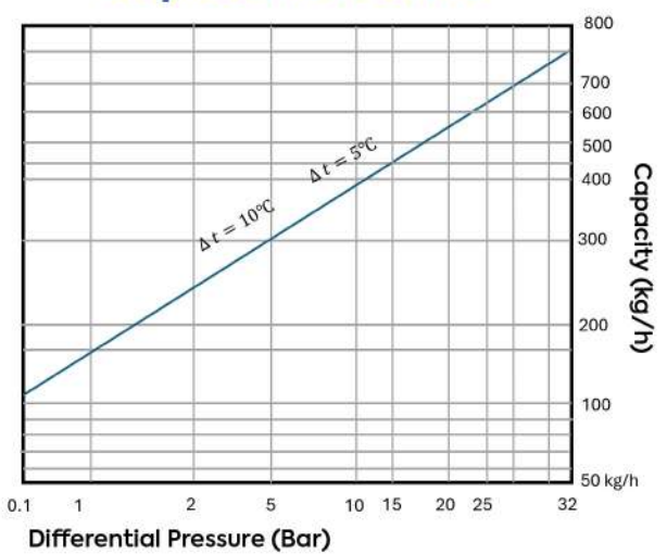
Displacement Curve
